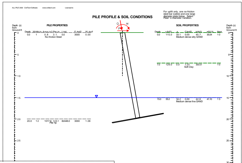
Plate in Deep Mode steel bar Figure 1
